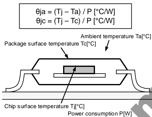
Fig.28 Thermal resistance
