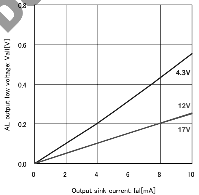
Fig.14 AL output low voltage (Ta=25°C)
