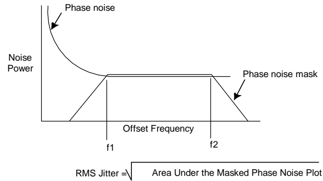
Figure 6. RMS Phase Jitter
