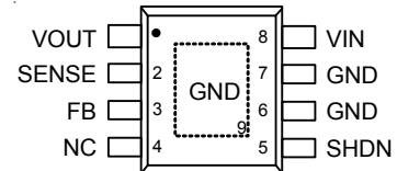
RT9068 SOP-8
