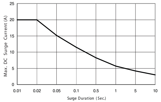
Figure 2. Surge Current Capability
