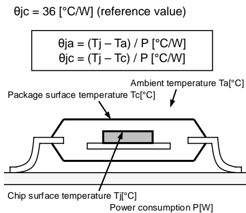
Fig.34 Thermal resistance
