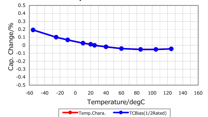
Temperature Characteristics
