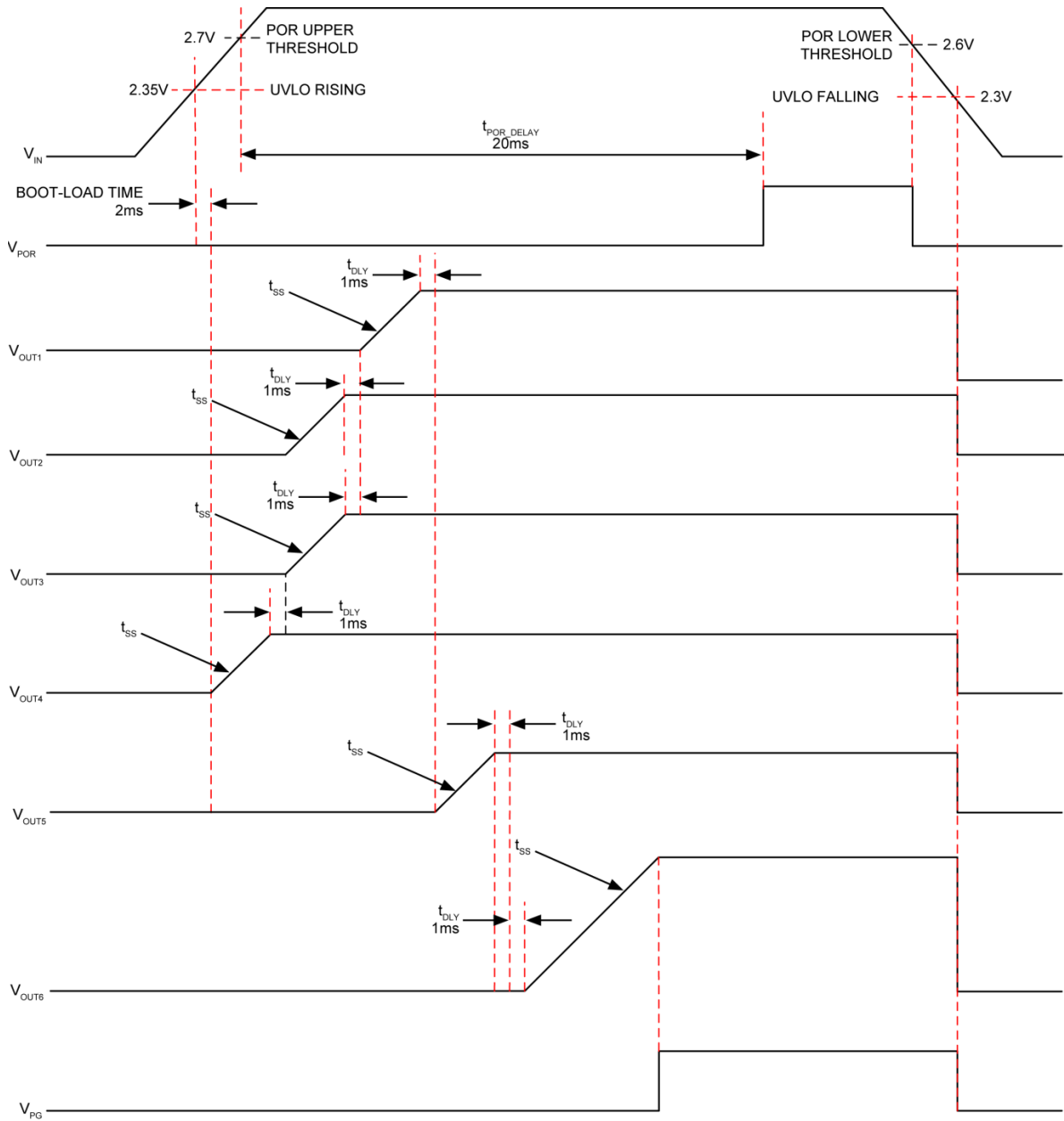
Figure 19. MIC7401 Power-Up/Down
