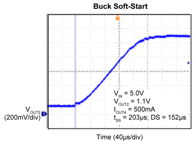
Figure 2. Buck Soft-Start
