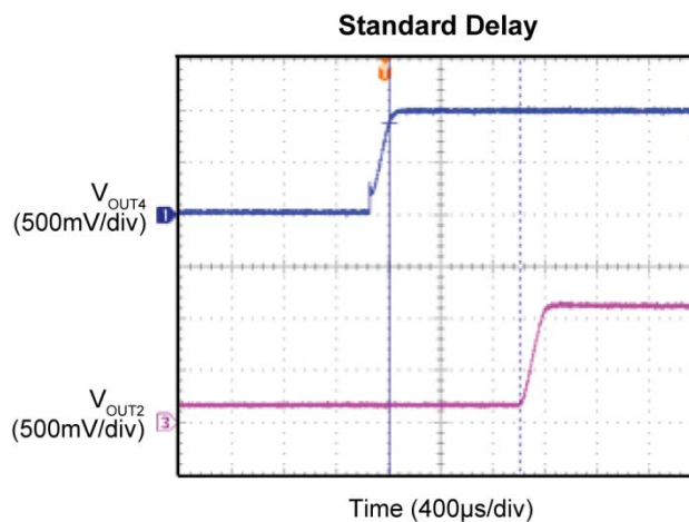
Figure 8. Standard Delay Time
