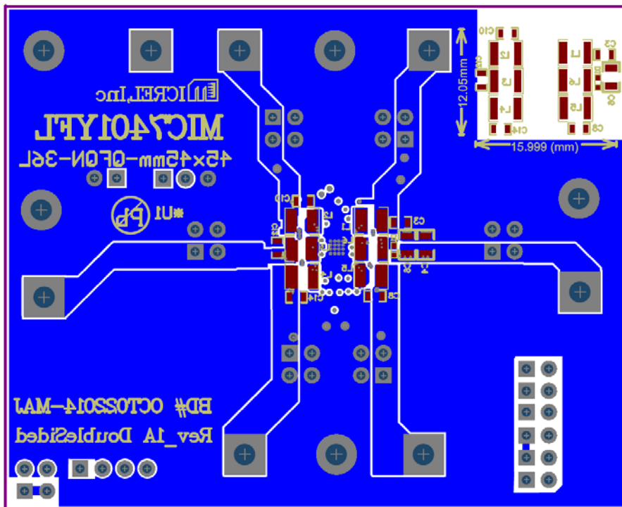
Evaluation Board Bottom Later – Layer 6 (Ground Plane)
