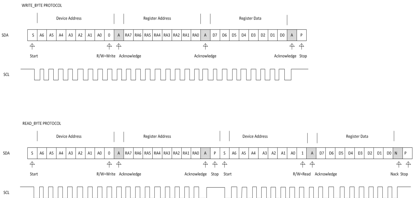
Figure 22. Read/Write Protocol
