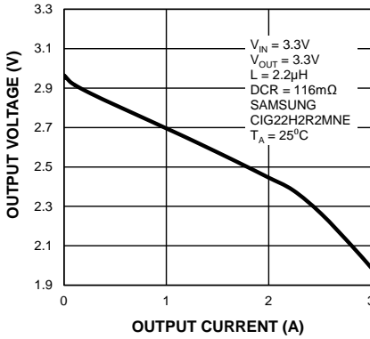
Dropout Output Voltage vs. Output Current
